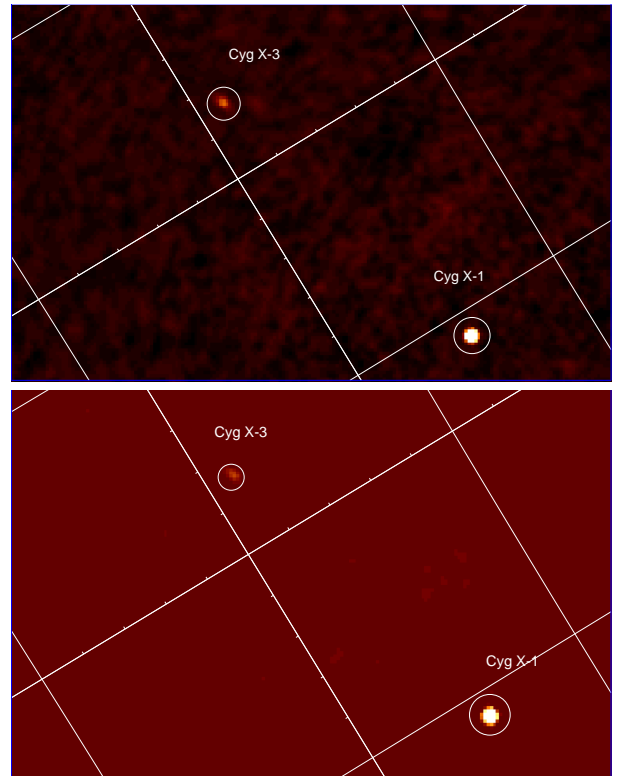
Fig. 1. 15-40 keV (top) and 40-100 keV deconvolution images of IBIS/ISGRI observations during revolution 16. They result from the sum of 56 Science Window of duration varying between 1800 and 3600 seconds for a total of \sim 147 ksec. The confidence levels start from 10 \sigma and are linearly spaced. The white grid represents Galactic Coordinates, the lines are spaced by 6 degrees. Cyg X-1 is at the bottom left and is detected at \sim 1000 \sigma and \sim 850 \sigma level respectively, Cyg X-3 is on top right at \sim 160 \sigma and \sim 55 \sigma level respectively
