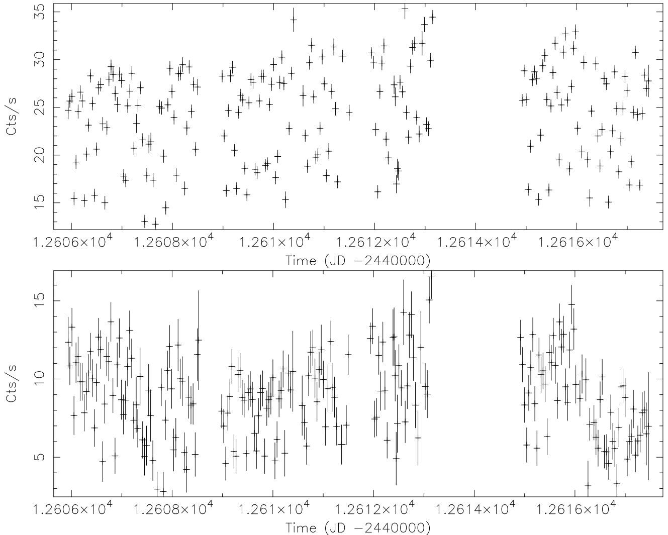
Fig. 2. Cyg X-3 15-40 keV (top panel) and 40-100 keV (bottom panel) light curves for revolutions 15 to 18. The horizontal time scale is in days. Each point represents a science window of duration varying between 1800 and 3600 seconds. Periodic gaps in the data are due to radiation belt passes while the longer gap at day 1.2614 \times 10^4 is due to a data loss. The point to point variation reflect the 4.8-hour modulation.
